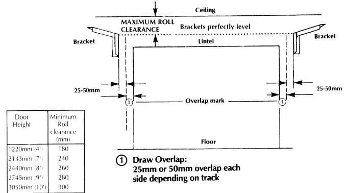
FIGURE 5 : FIX BRACKETS
